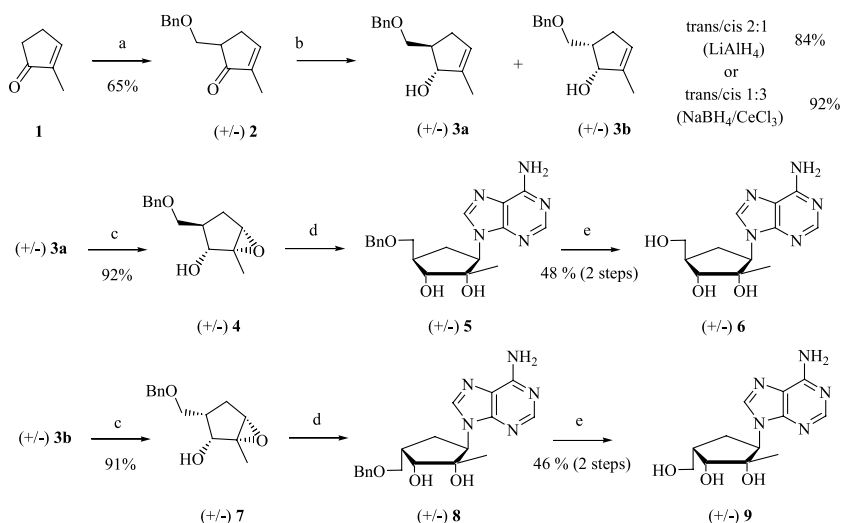
SCHEME 1 Reagents: (a) Lithium diisopropylamide (LDA), benzylbromomethyl ether, THF, -78 to -50^{\circ}\text{C} ; (b) LiAlH 4 , ether, -78 to -60^{\circ}\text{C} or CeCl 3 ·7 H 2 O, NaBH 4 , MeOH, 0^{\circ}\text{C} ; (c) 3-chloroperoxybenzoic acid ( m -CPBA), methylene chloride, 0^{\circ}\text{C} ; (d) NaH, adenine, DMF, 100^{\circ}\text{C} ; (e) palladium hydroxide on charcoal, cyclohexene, MeOH, reflux.
