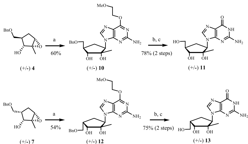
SCHEME 2 Reagents: (a) NaH, 2-amino-6-(methoxyethoxy)-purine, DMF, 120°C; (b) 3N HCl, dioxane, 80°C; (c) palladium hydroxide on charcoal, cyclohexene, MeOH, reflux.
